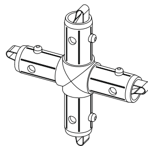
TC-30-X 4-way cross connector
